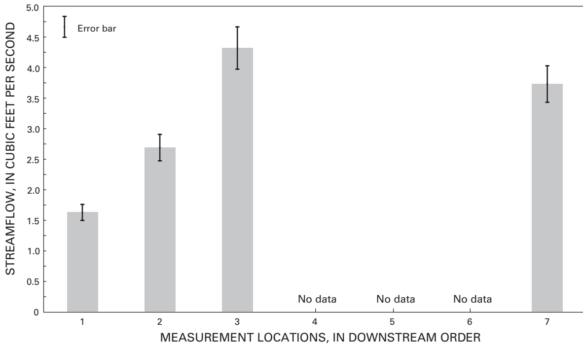
Figure 12. Comparison of streamflow among measurement locations from Brooks (1983), October 5, 1982, Terror Creek, Colo., water year 2003.
