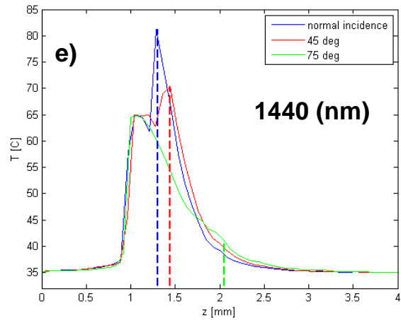
Fig. 18: Analysis of the fat/dermis border on thermal effects. At close distance ( D = 0.5 mm) of the lipolysis cannula to the fat/dermis border, the thermal effect in the dermis is smallest with the 1064 nm laser. At other wavelengths, the thermal effects are more expressed and can exceed the maximal allowed temperatures. The largest undesired thermal effect in the dermis is with the 1440nm.
